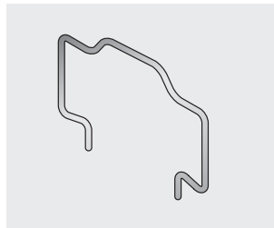
Shadow Gap Edge Trim No. 6 Can be delivered concave or convex Size: 20 × 38 × 14 × 4000 mm Skygge: 6 × 9 mm Material: Galvanised steel Finish: Painted
